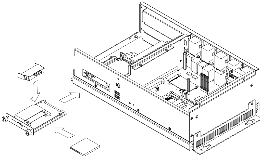
Figure 3.6 Installing the CF Card Module
