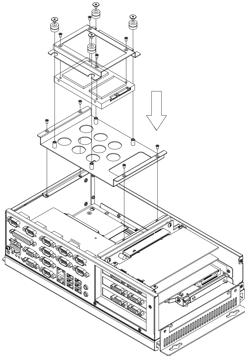
Figure 3.3 Installing the HDD Module
