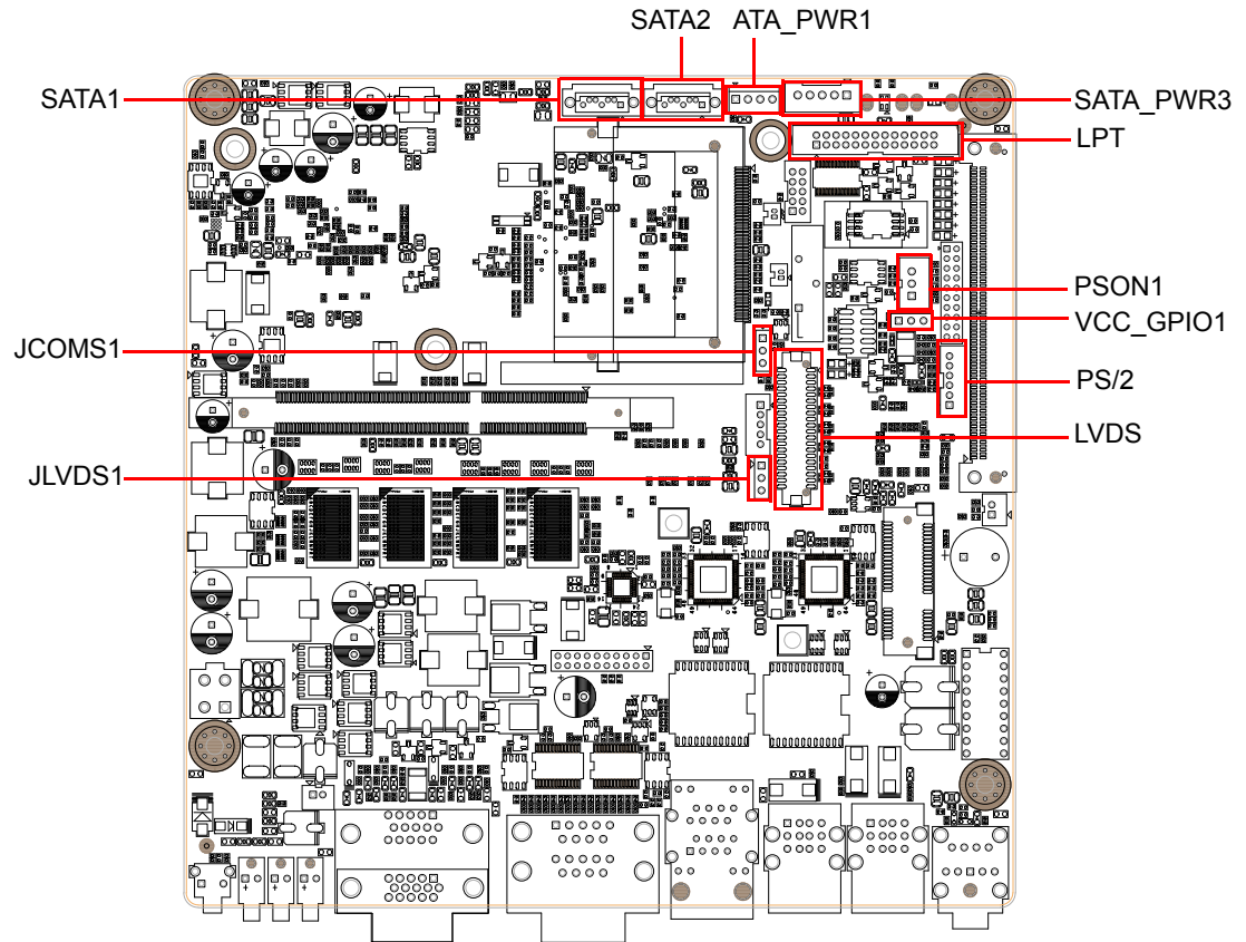
Figure 2.2 Jumper and connector location
