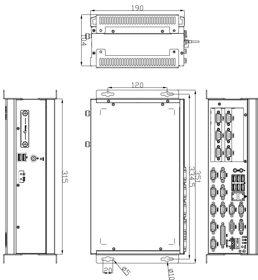
Figure 1.1 Dimension Diagram of ITA-1910
