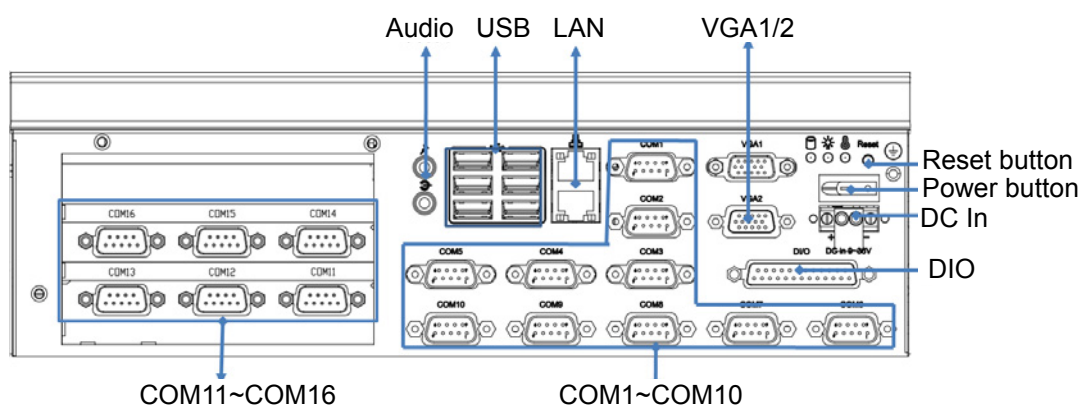
Figure 2.6 ITA-1910 Rear I/O Connectors
