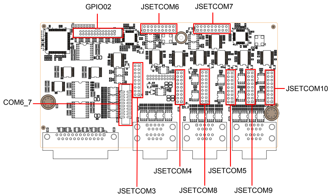
Figure 2.3 Jumper and connector location of expanded 8COM I.O board
