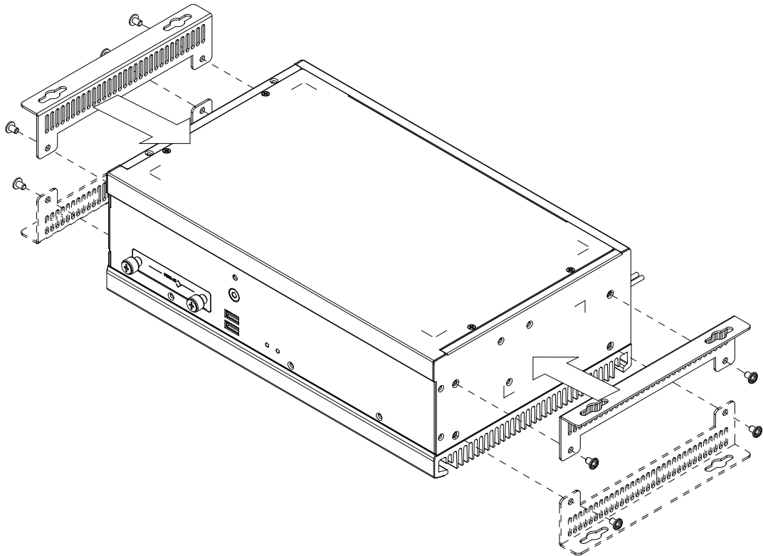
Figure 3.5 Installing the Foot Stand
