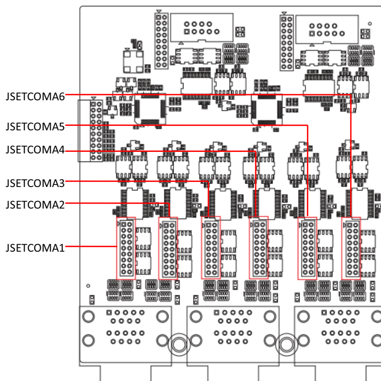
Figure 2.4 Jumper location of expanded 6 COM I.O board
