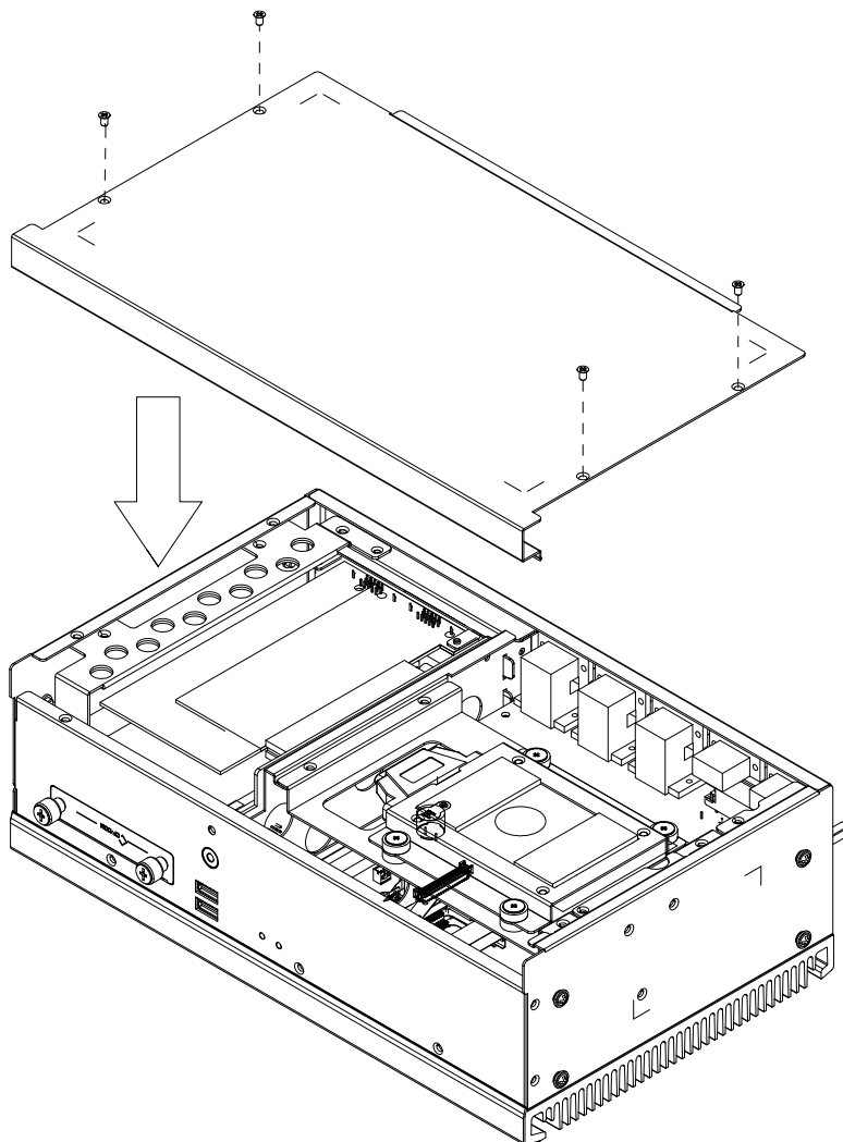
Figure 3.4 Installing the Top Cover
