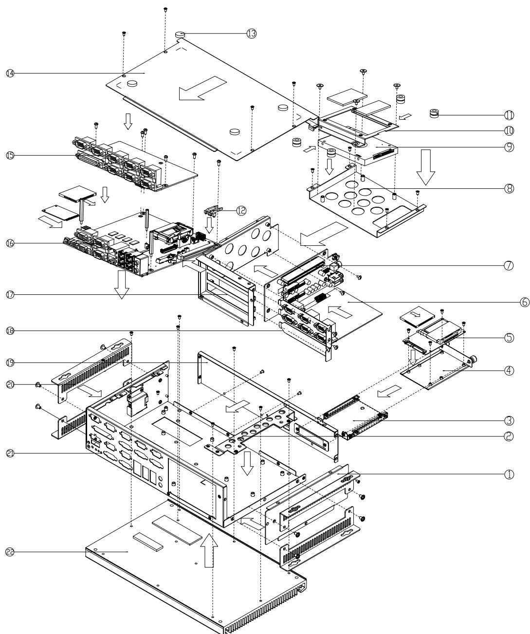
Figure 1.2 Exploded Diagram of ITA-1910
