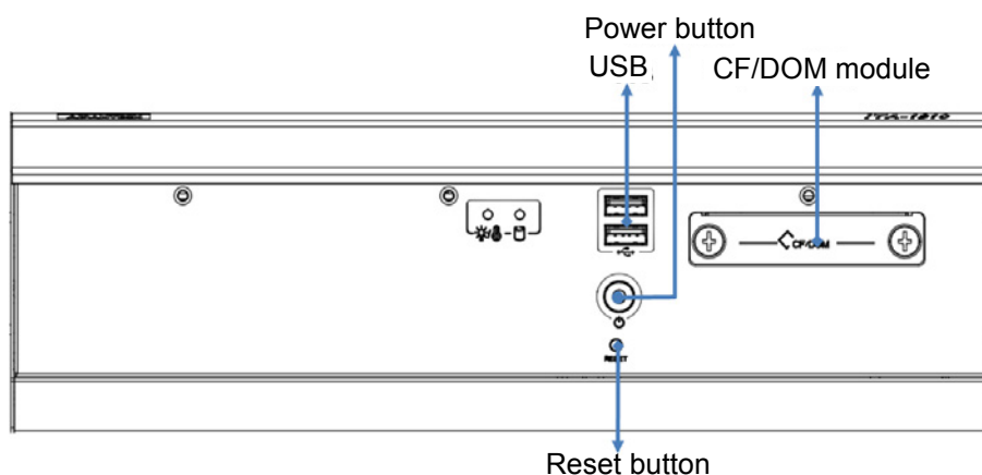
Figure 2.5 ITA-1910 Front I/O Connectors
